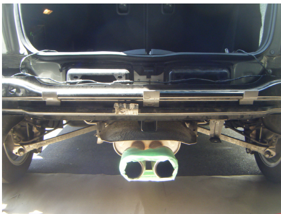
Photo 9: Hitch and bumper beam installed
