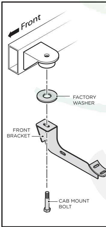
Front Bracket
