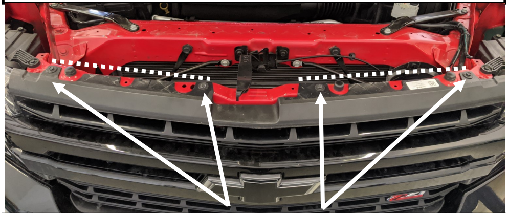
Figure 3: Grille removal.
