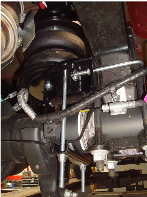
Passenger's (right) side installation from the rear
