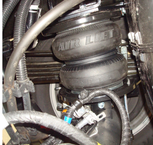
Driver's (left) side installation from the middle
