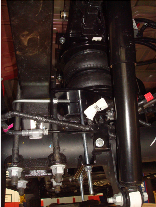
Driver's (left) side installation from the rear
