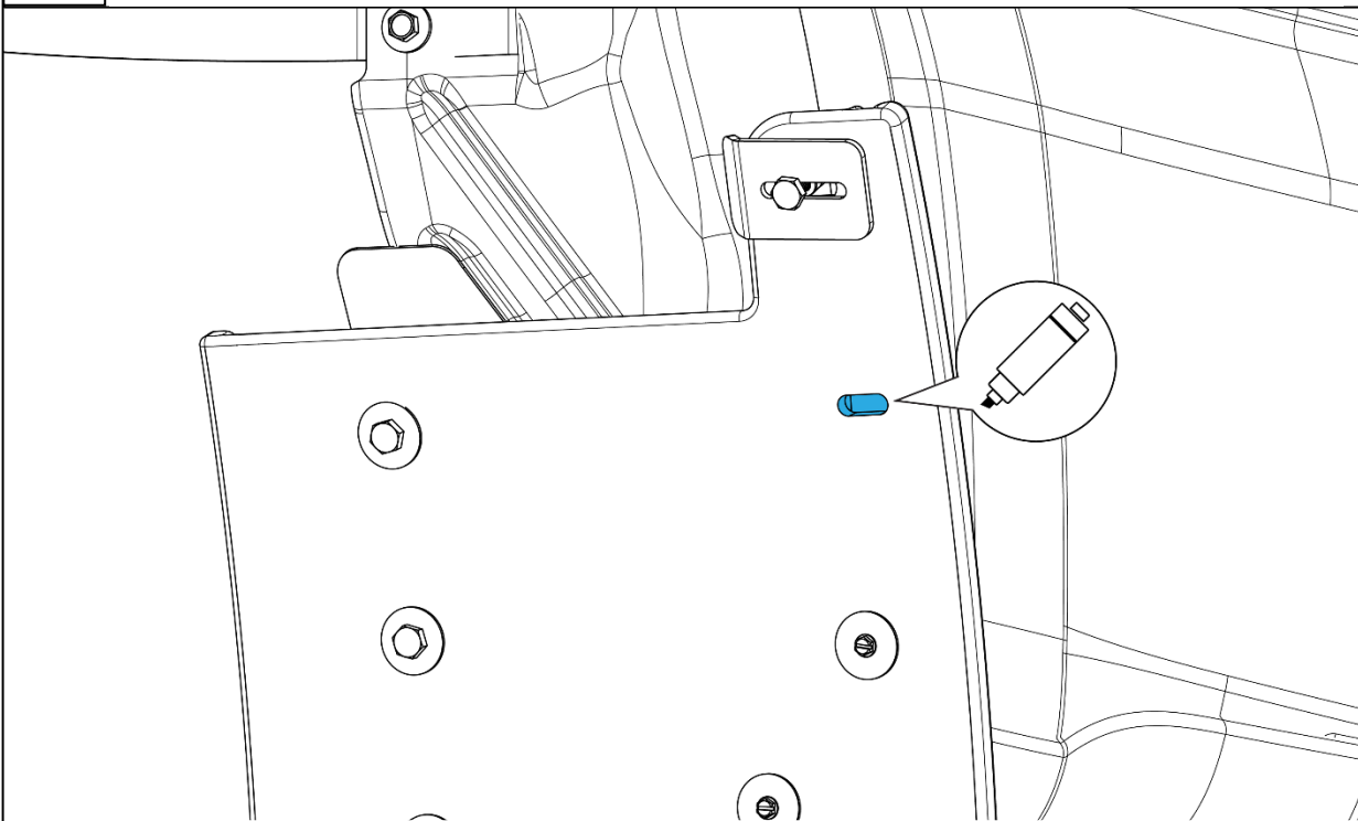
9-1 With the mud flap held tight to the fender lip, mark the fender through the remaining mud flap hole. This provides a guide for installing the protective tape and spring nut as shown in 9-2.
