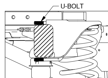
Figure E2: Cutaway view of suspension spring area looking towards the rear of the truck
