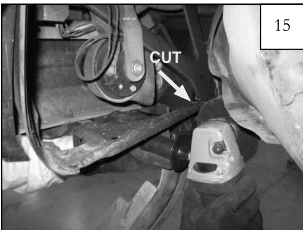
Carefully cut lower sheet metal strut attached to fender.
