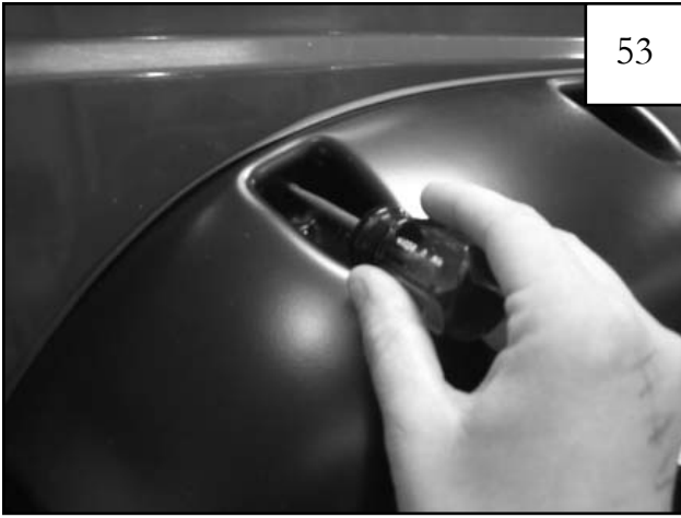
Using the holes in the part as a guide, mark hole locations on fender (4 places).
