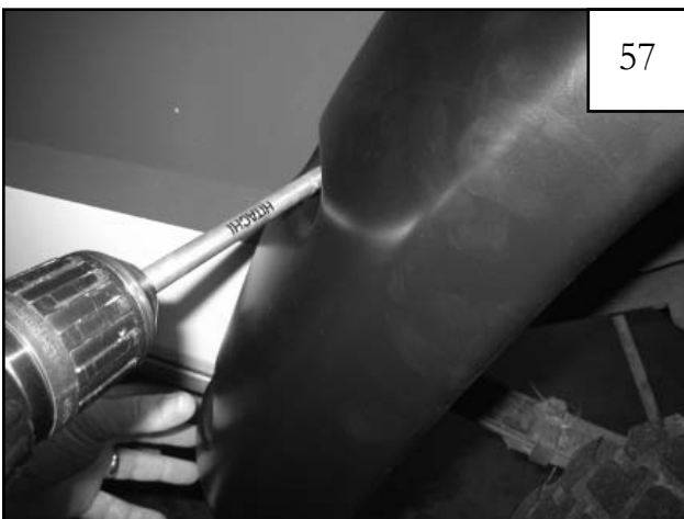
Start each screw with a T45 Torx bit in each pocket but do not tighten until all screws have been started. Over-tightening screws may cause them to strip! Use a Torque setting of 24 inch/ounces.
